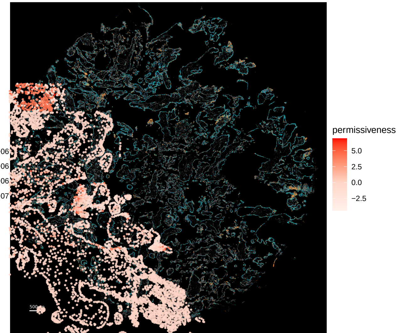
starmap_with_permissiveness W8-2 (white->red overlay)
